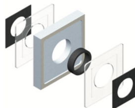
Plaque de support 260 x 260
